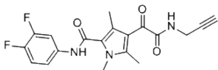
PC-3525401, Acetone-d 6
